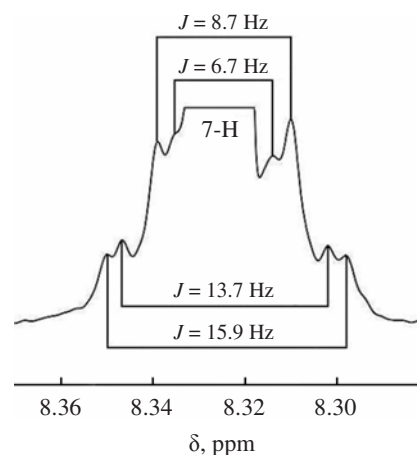
Fig. 2. Fragment of the ^1H NMR spectrum of triazolothiazine IIIa ( IVa ).
