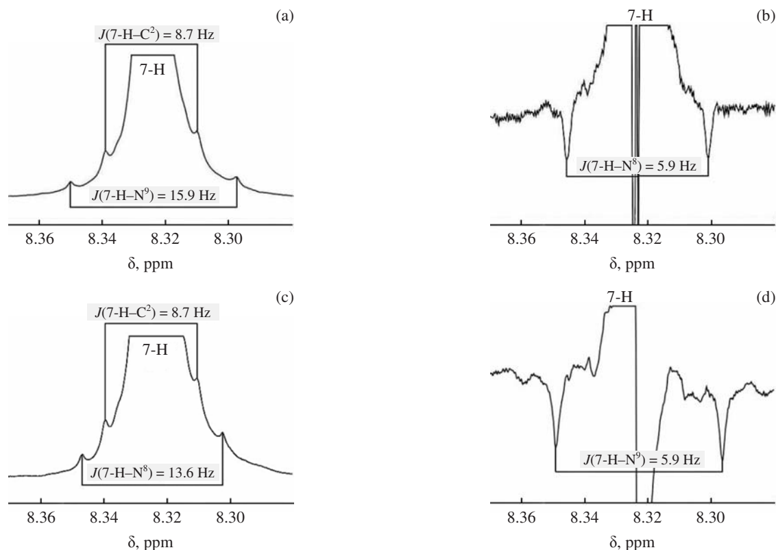
Fig. 4. Fragments of (a, c) conventional and (b, d) difference ^1\text{H} NMR spectra of triazolothiazine IIIa ( IVa ), recorded with selective decoupling from (a, b) \text{N}_\text{pn}^8 and (c, d) \text{N}_\text{pn}^9 .
